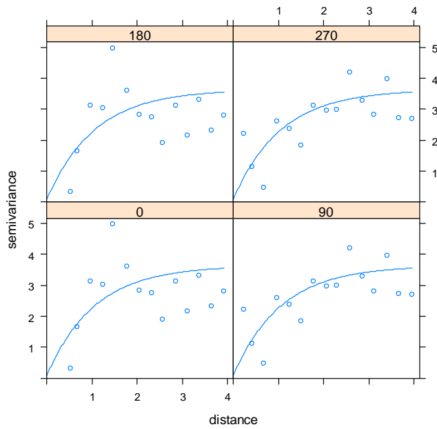
Figure 3-13: West Nile Virus Anisotropic Variogram for California
